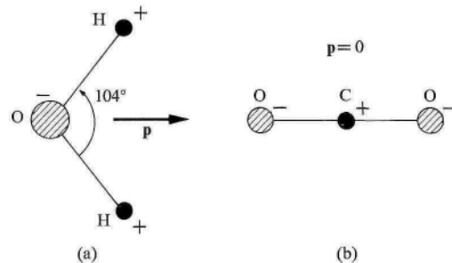
Fig.4.1 (a) The water molecule (b) CO 2 molecule.
